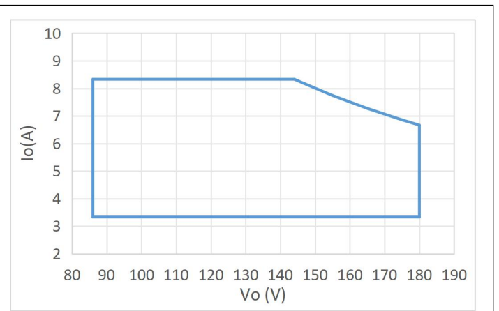
Figure 5.I/V Operating Area (1200HTH180CV)
