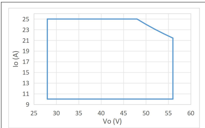
Figure 4.I/V Operating Area (1200HTH56CV)
