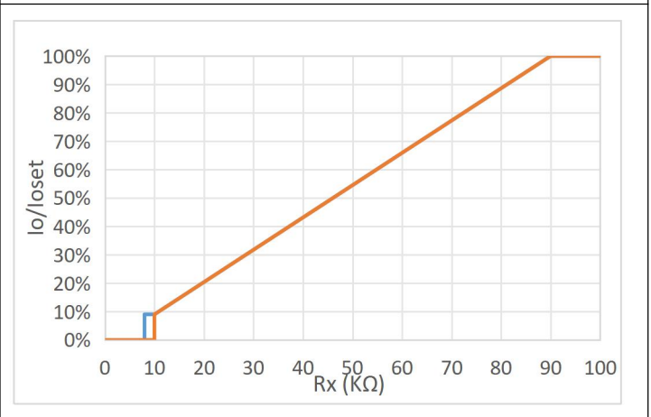
Figure 15. I_o/I_{oSet} vs R_x
