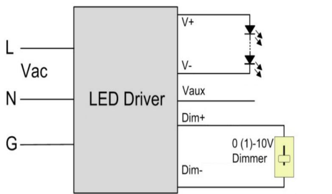
Figure 10.The Block Diagram of 0-10V Analog Dimming
