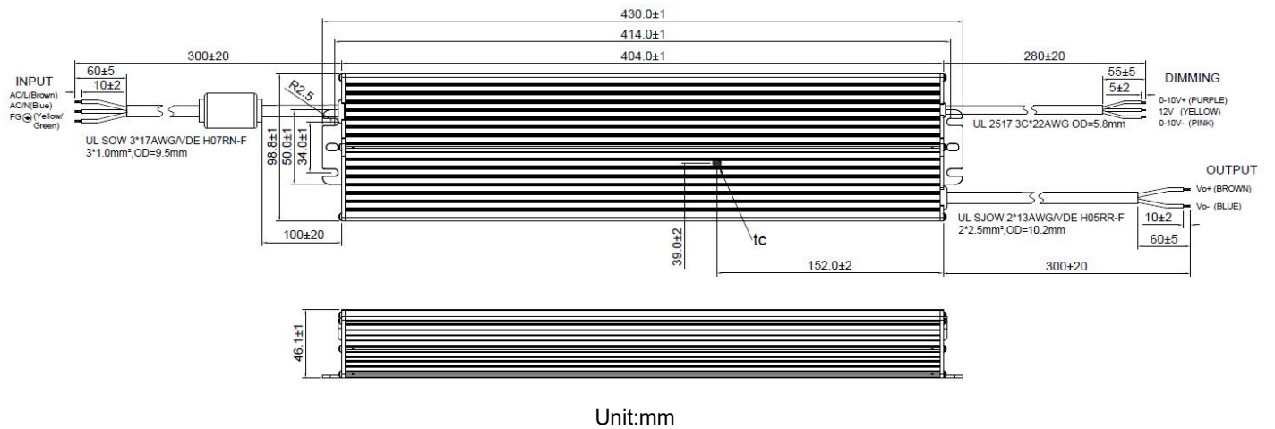
Figure 17. Mechanical Drawing
