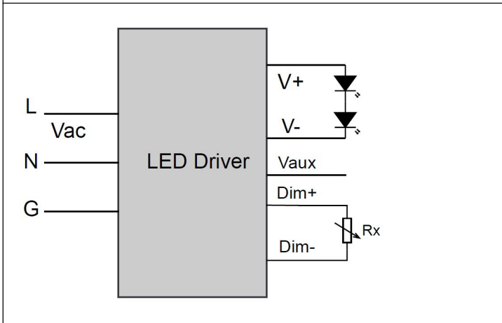
Figure 14. The Block Diagram of Resistor Dimming
