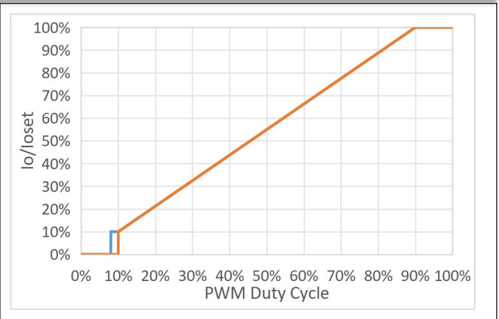
Figure 13. I_o/I_{oSet} vs PWM Duty Cycle
