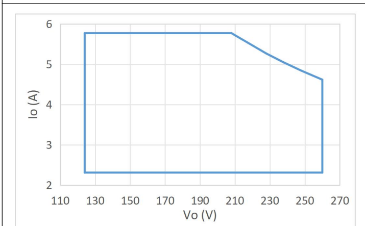
Figure 6.I/V Operating Area (1200HTH260CV)
